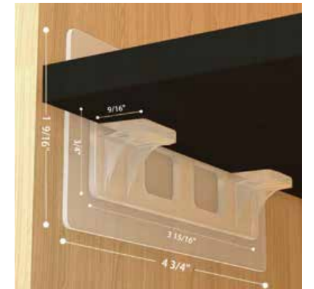
Angled Support Bracket
